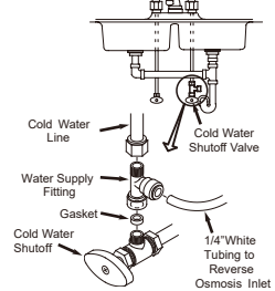
Cold Water Supply Connection (using included water supply fitting)
